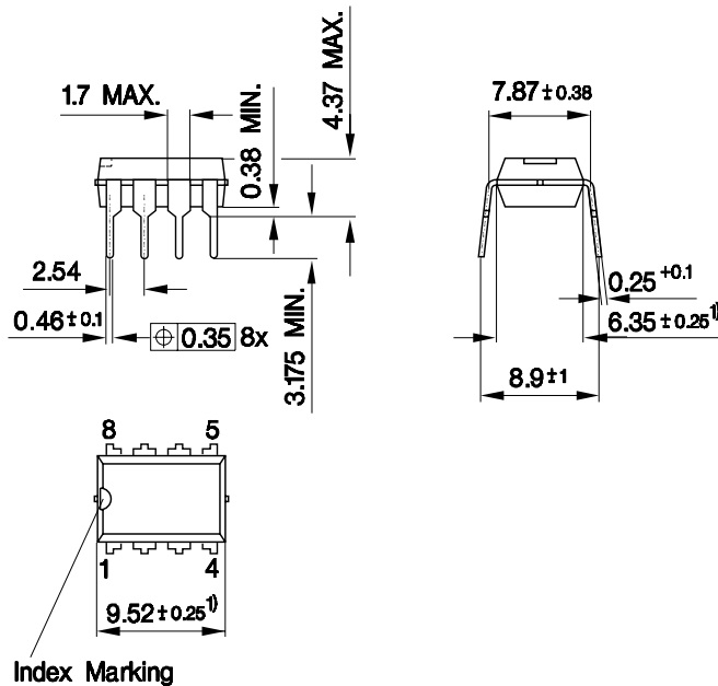
Figure 22 PG-DIP-8-6 ( Pb-free lead plating Plastic Dual-in-Line Outline )
